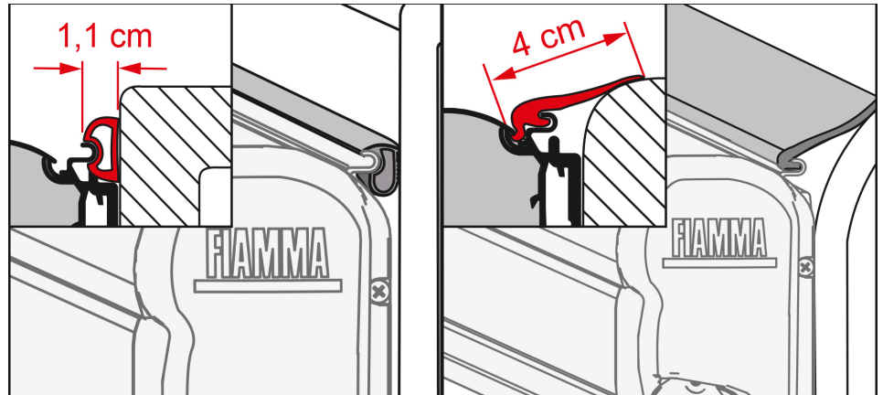
Rain Guard S
